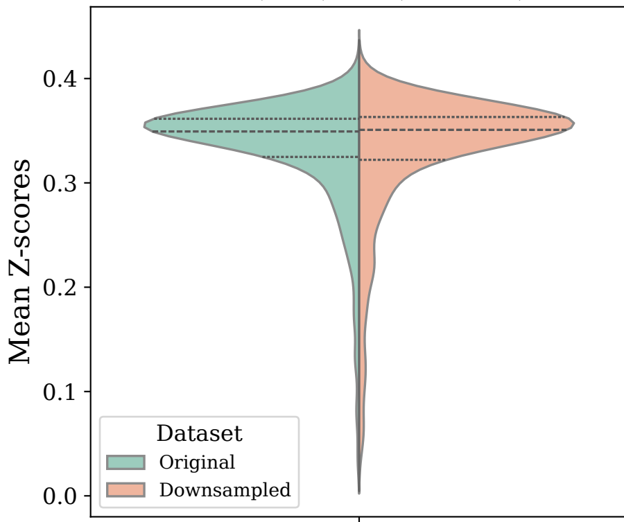
Distribution of Mean Z-scores Original N=100 vs Downsampled N=100k to R=100 \sigma = (1, 1) v = (0.1, 0.5)
